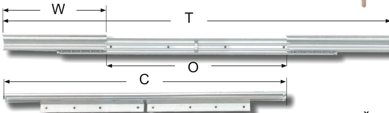
In mm Model Top Slide 9097 Steel - Zinc Plated
